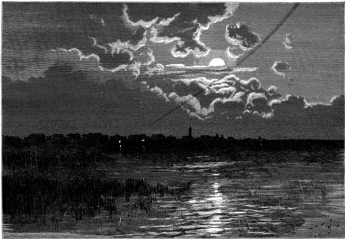
Sl. 46. Delta (Raztok).
